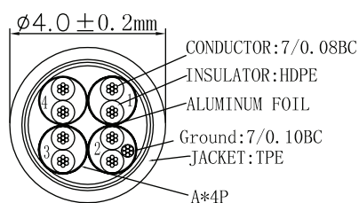
SECTIONAL DRAWING:
