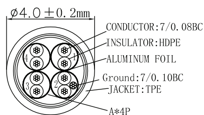
SECTIONAL DRAWING:
