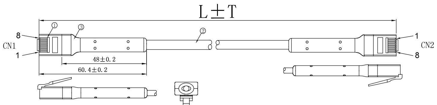
SECTIONAL DRAWING:
