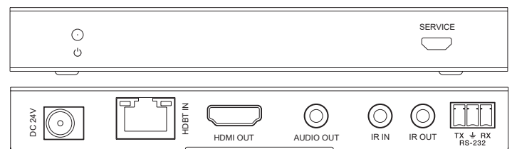
Receiver
