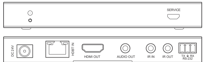
Receiver Panel
