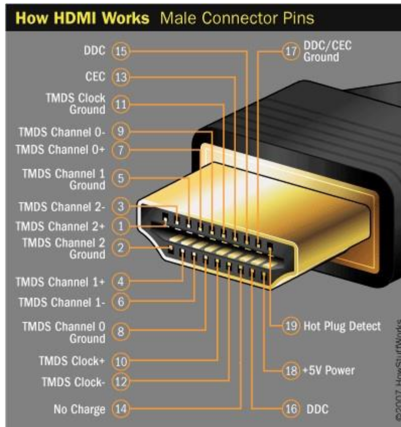
Figure 1 - HDMI Under the Hood
